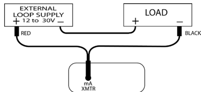
Fig 3. Simulate a 2-Wire mA Transmitter Loop With External 12 to 30V DC Supply. A similar connection can be used to extend output range of CVC beyond 300 ohms. A 24V source will allow CVC to source into an impedance of >1000 ohms.
